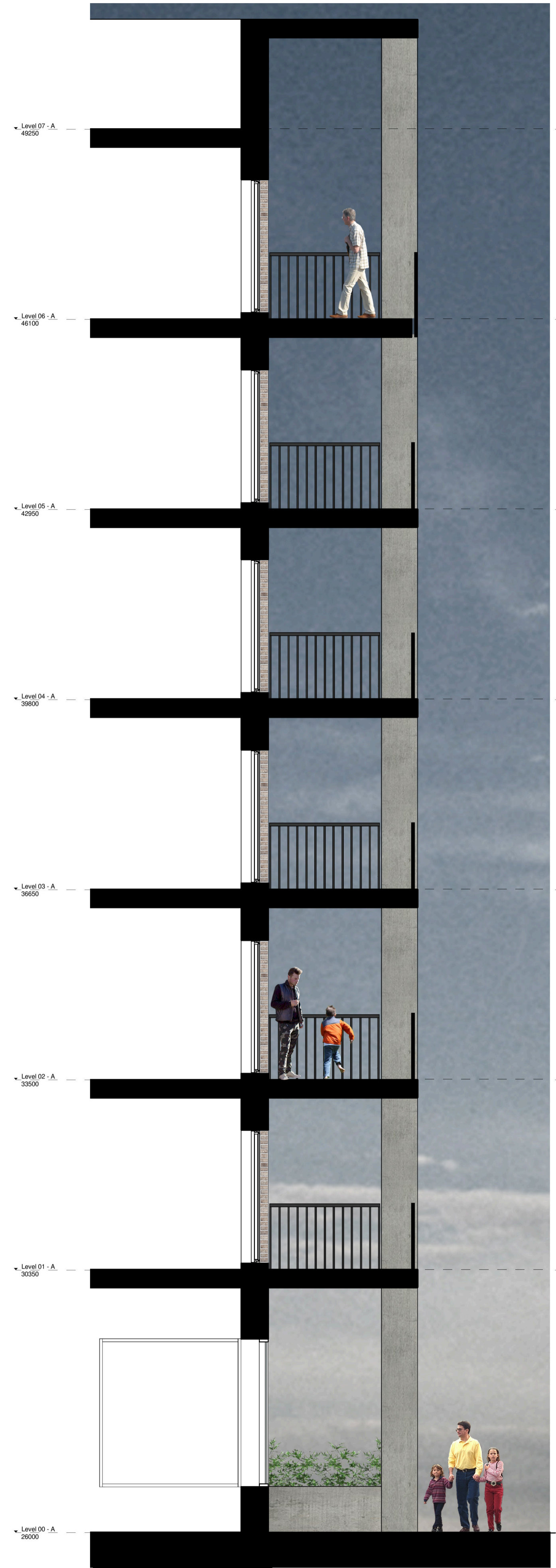
2 Block G Study Section 1:50
